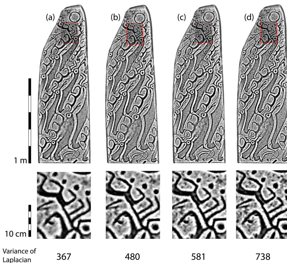
Fig. 4. Effect of model resolution, using stela #35 as an example, with the volumetric obscurity-based approach. Number of faces tested: 250,000 (a), 500,000 (b), 1 M (c) and 2 M (d). From top to bottom: projection of one side after processing the entire stela, a close-up corresponding to the red inset, the value of the variance of Laplacian computed from the projection (For interpretation of the references to colour in this figure legend, the reader is referred to the web version of this article).
