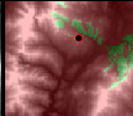
MNT + Viewshed
